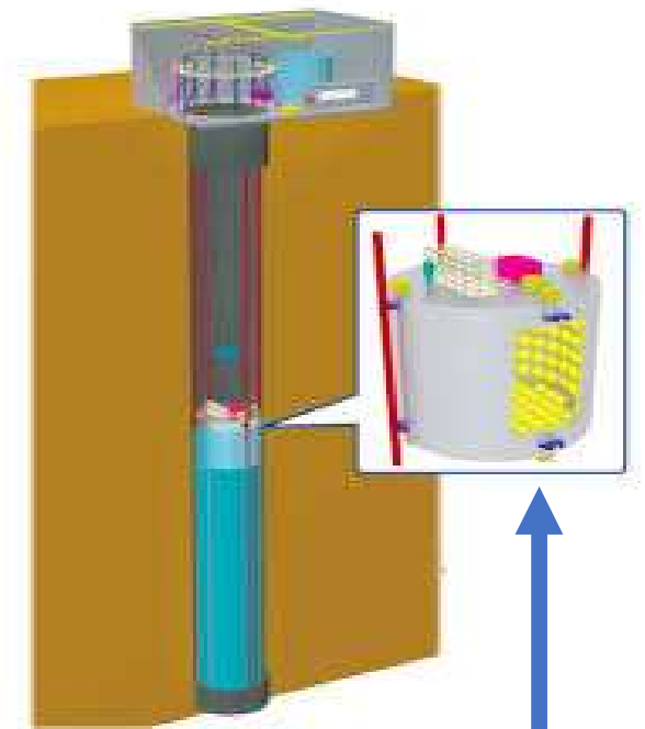
Water Cerenkov detector
