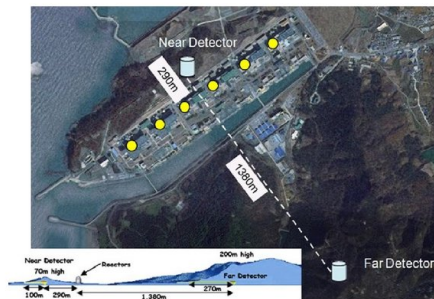
Figure 7: Detector locations and design in RENO experiment [11].
