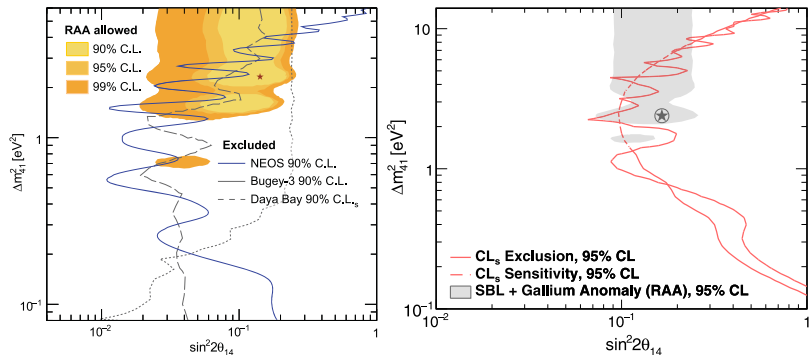
Figure 10: NEOS (left plot, 2017, [16]) and PROSPECT (right plot, 2021, [17]) results on sterile neutrinos.
