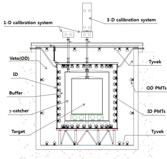
Figure 7: Detector locations and design in RENO experiment [11].
