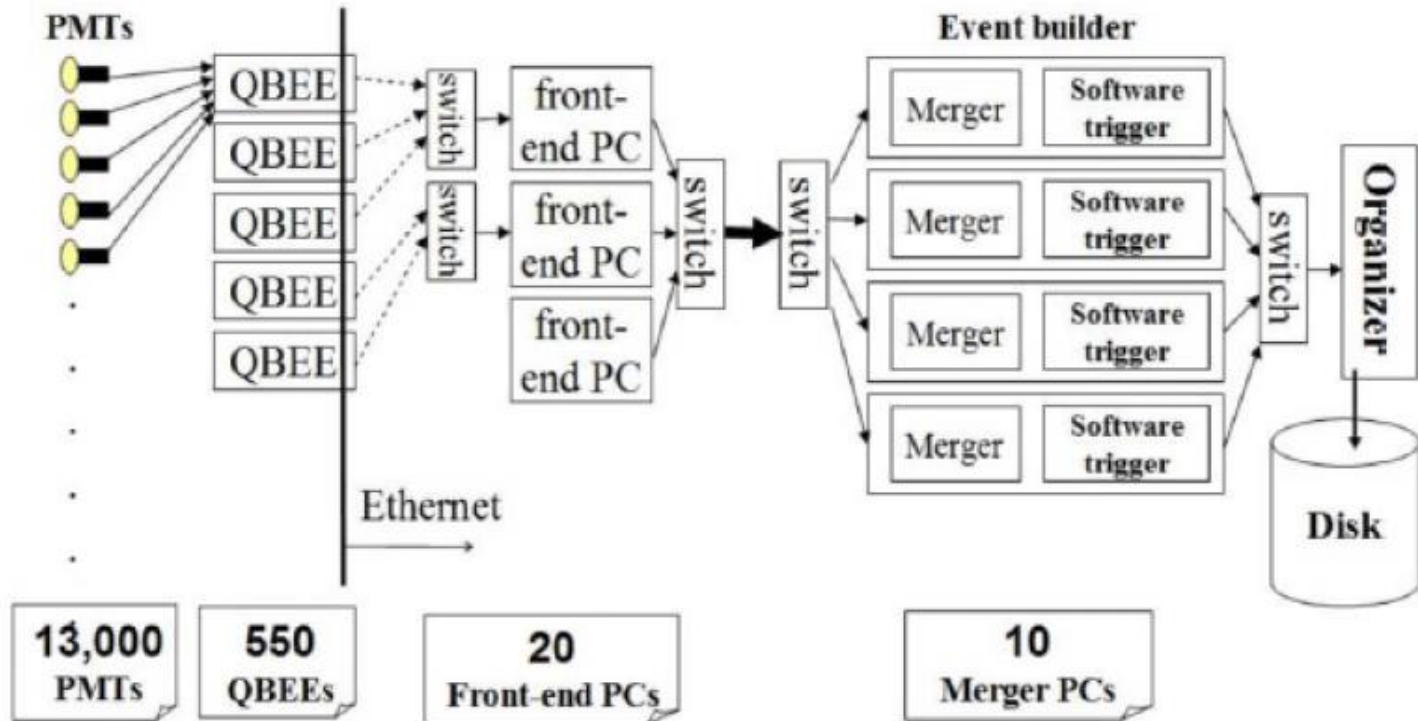
Figure 3.10: The schematic view of the DAQ system used in SK-IV [97].
